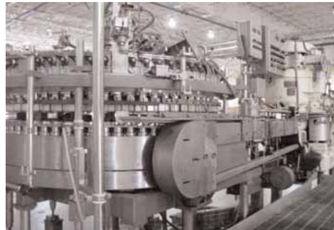
CC&S 72-Valve Can Filler & Angelus Can Seamer
