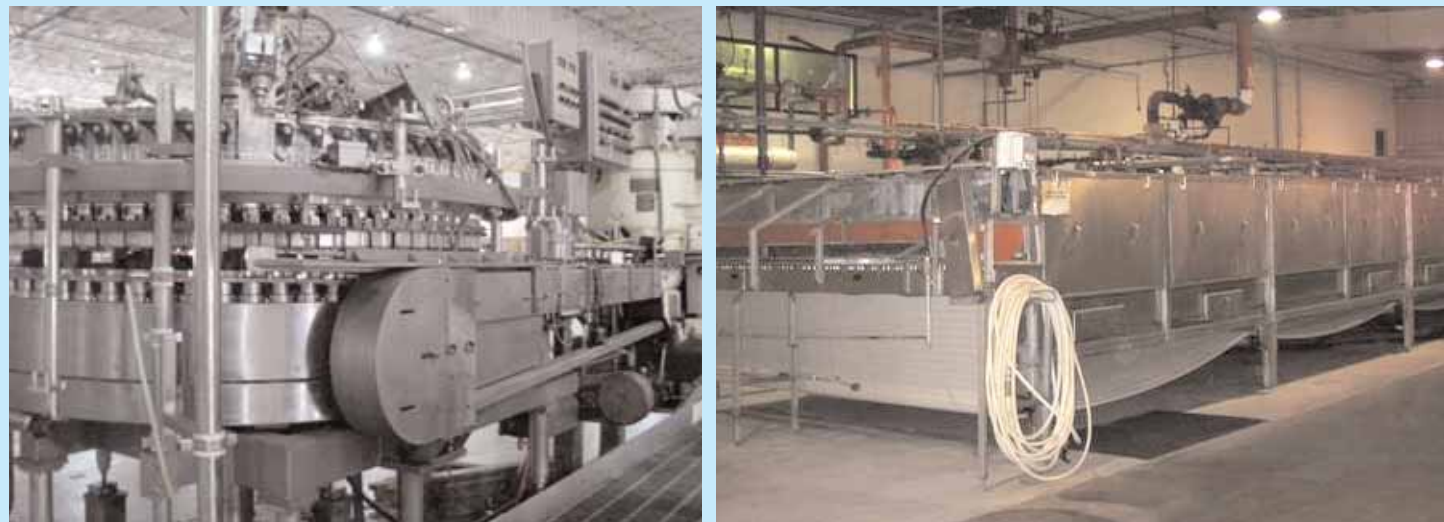
CC&S 72-Valve Can Filler & Angelus Seamer - Aeroglide Pasteurizing/Cooling Tunnel
