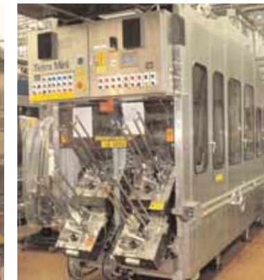
Tetra Pak Rex Model TR-6 Carton Filler with Fitment and Tetra Mini Half-Pint Carton Filler
